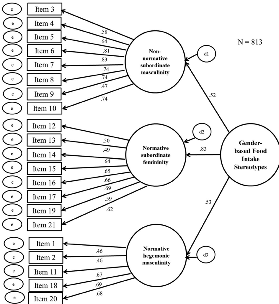
Figure 2. Note: \chi^2(186) = 618.65, p < .001, \chi^2/df = 3.32, CFI = .92, RMSEA = .053, 90\% CI [.049; .058] . Coefficients are standardized. No item-factor loading was below the recommended level of \beta = .30 (Kline, 2016). Loadings were all significant ( p < .001 ).
