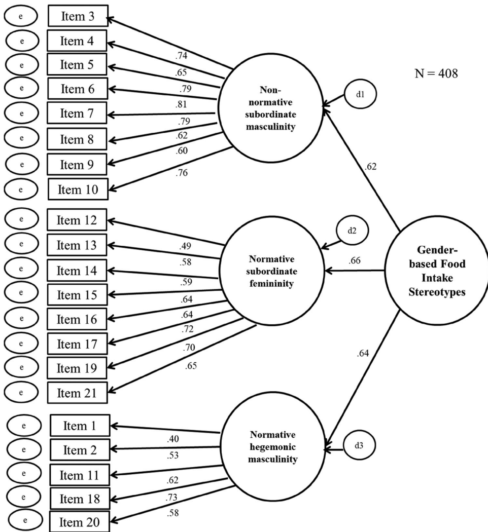
Figure 1. Note. Fit model: \chi^2(186) = 457.27, p < .001, \chi^2/df = 2.46, CFI = .91, RMSEA = .060, 90\% CI [.053; .067] . Coefficients are standardized. No item-factor loading was below the recommended level of \beta = .30 (Kline, 2016). Loadings were all significant ( p < .001 ).
